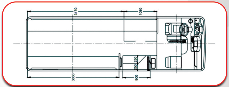
SEAT LAYOUT
