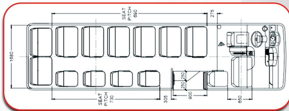
SEAT LAYOUT
